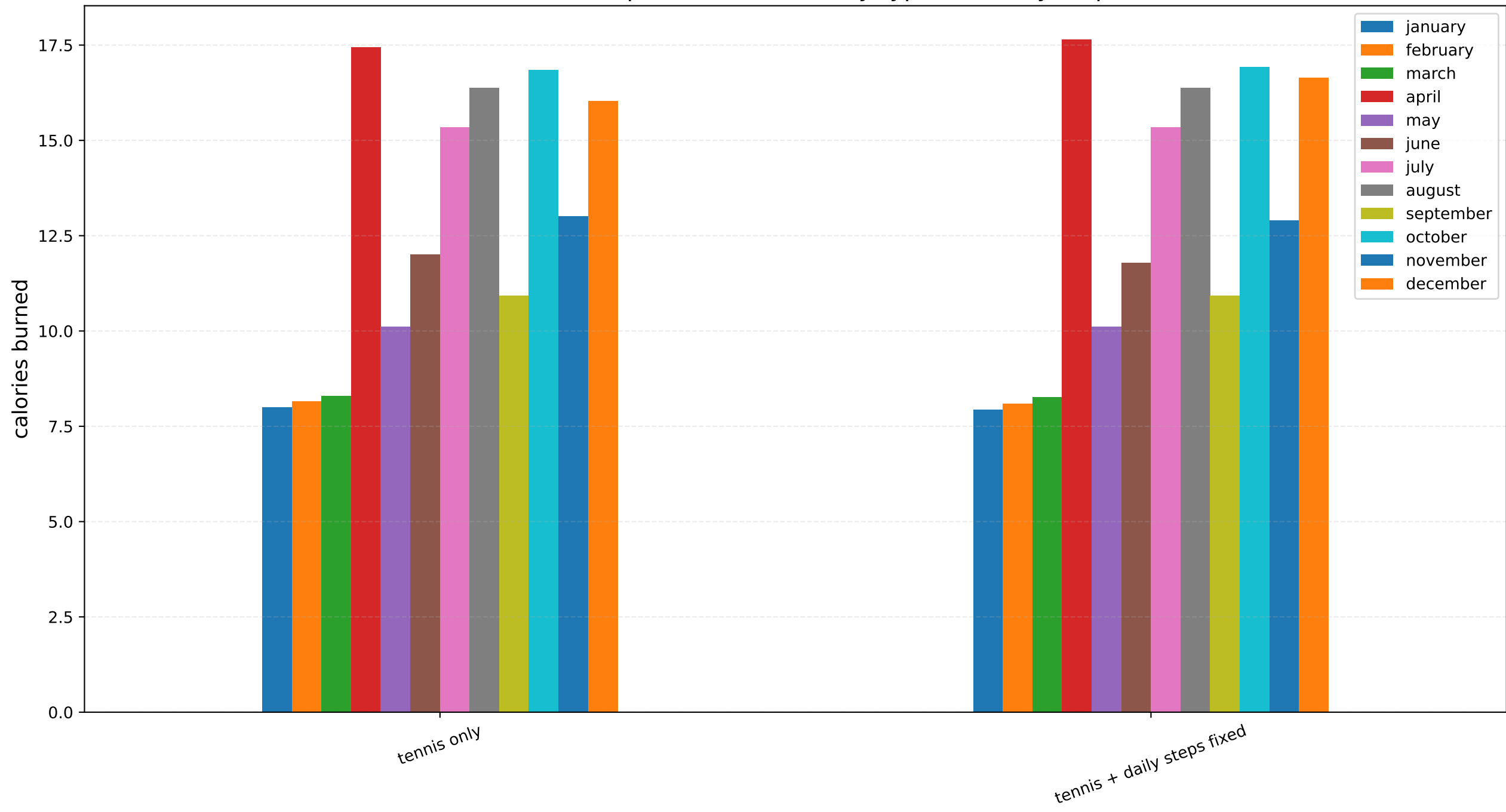
Counterfactual outputs: PID=6, activity type and daily steps fixed
